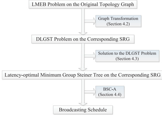
Fig. 4. Overview of solution to the LMEB problem.
