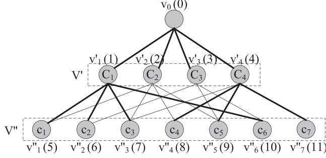
Fig. 20. An instance of the LMEB problem with L = 12 . Given an optimal broadcasting schedule M = \{M(v_0) = (1, \langle v'_1, v'_2, v'_3, v'_4 \rangle), M(v'_1) = (1, \langle v''_1, v''_2, v''_3, v''_6 \rangle), M(v'_4) = (1, \langle v''_4, v''_5, v''_7 \rangle), M(v'_2) = M(v'_3) = M(v'_j) = (0, \text{NULL}) (j = 1, \dots, 7)\} , we can easily get the optimal solution of the Set Cover Problem , that is, \{C_1, C_4\} .
